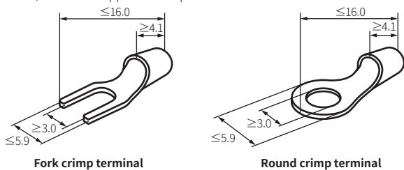
Fork crimp terminal
